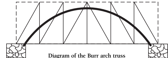
Diagram of the Burr arch truss
